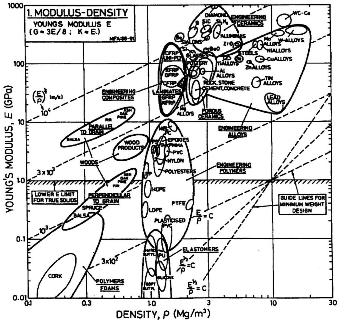
Relative position of materials comparing Young's modulus with density (Reference: M. F. Ashby. Materials Selection in Mechanical Design . Pergamon 1992)
