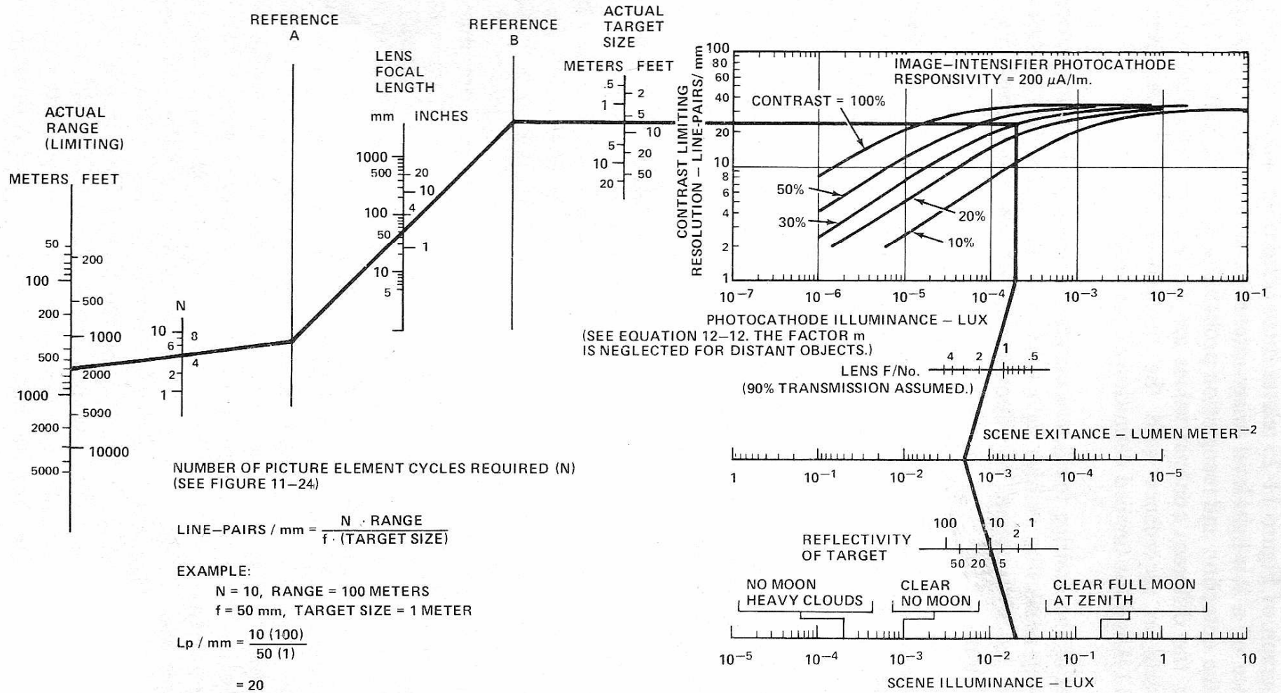
Nomograph for determining performance parameters of a low-light-level image intensifier target detection or recognition system.
